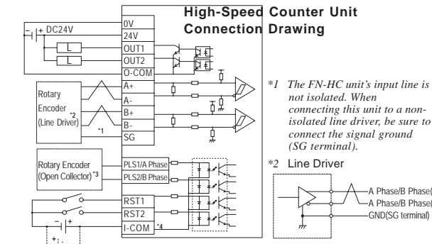
*3 Open Collector (Sink Output) Open Collector (Source Output)
